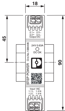
Dimensional drawing
