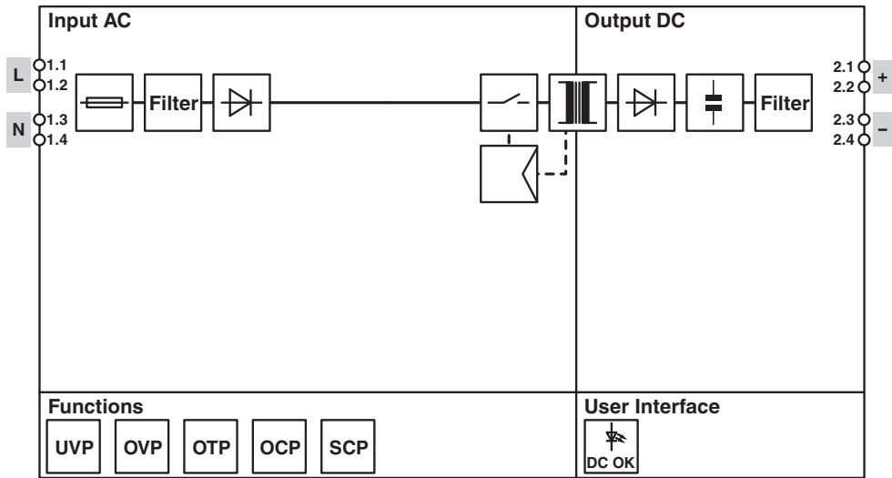
Block diagram
